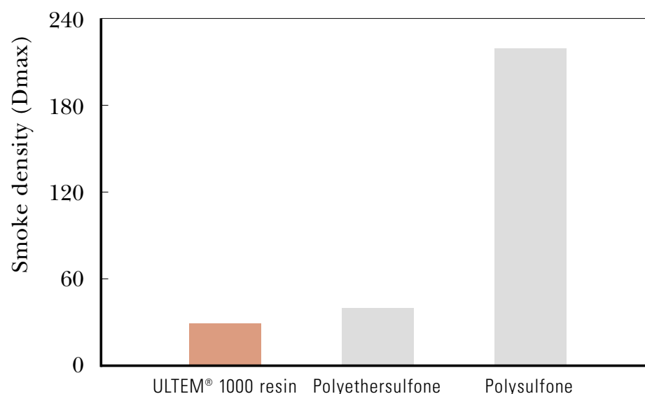
Smoke evolution by NBS test Dmax 20 min
