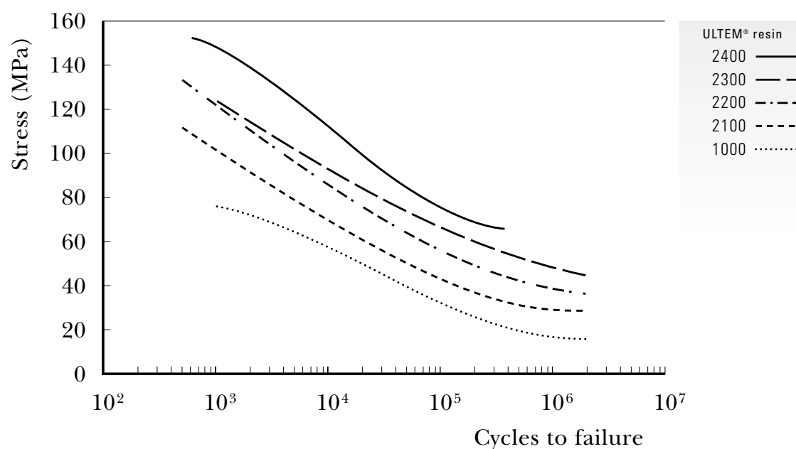
■ FIGURE 4-10 Uniaxial fatigue test of ULTEM® resin at different glass ratios
