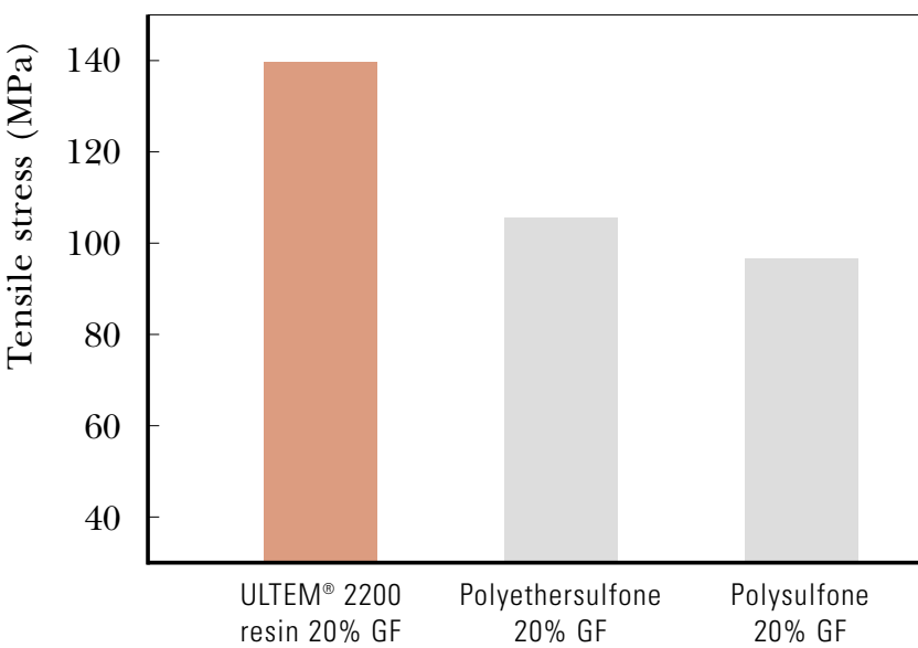
FIGURE 4-7 Tensile stress (23°C) at break (5mm/min)
