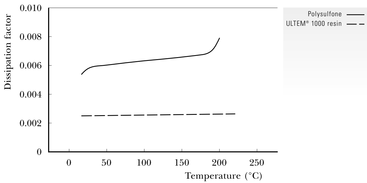
FIGURE 4-15 Dissipation factor vs. temperature at 2.45 \times 10^9 Hz
