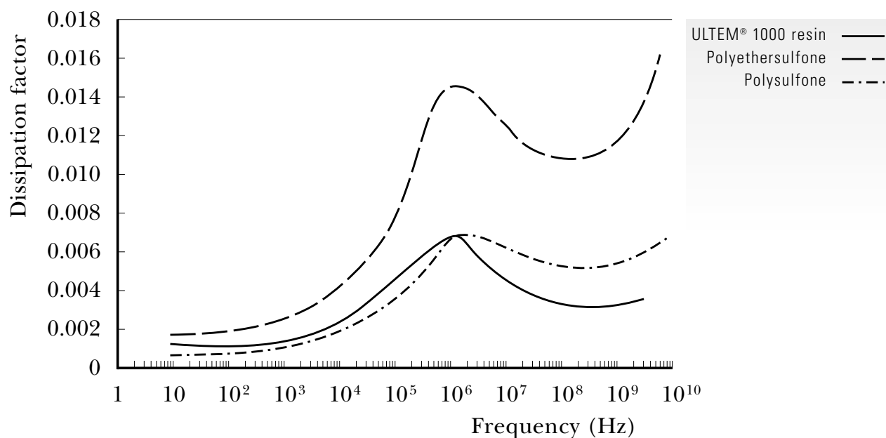
FIGURE 4-14 Dissipation factor vs. frequency at 23°C, 50% RH
