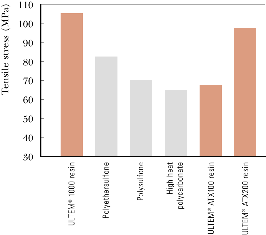
FIGURE 4-6 Tensile stress (23°C) at yield (50mm/min)
