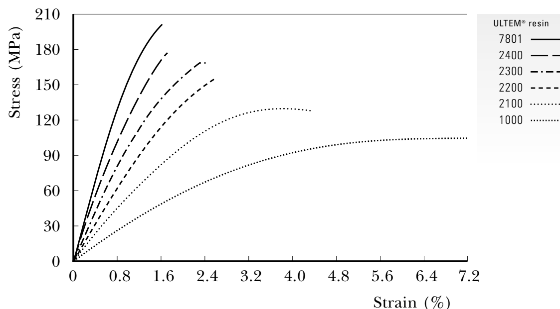
■ FIGURE 5-1 Stress-strain curve (23°C)
