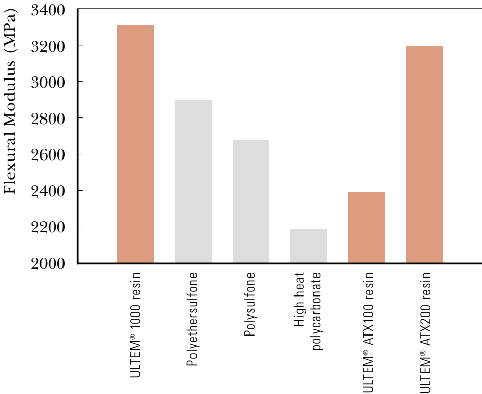
■ FIGURE 4-9 Flexural modulus (23°C) 2 mm/min
