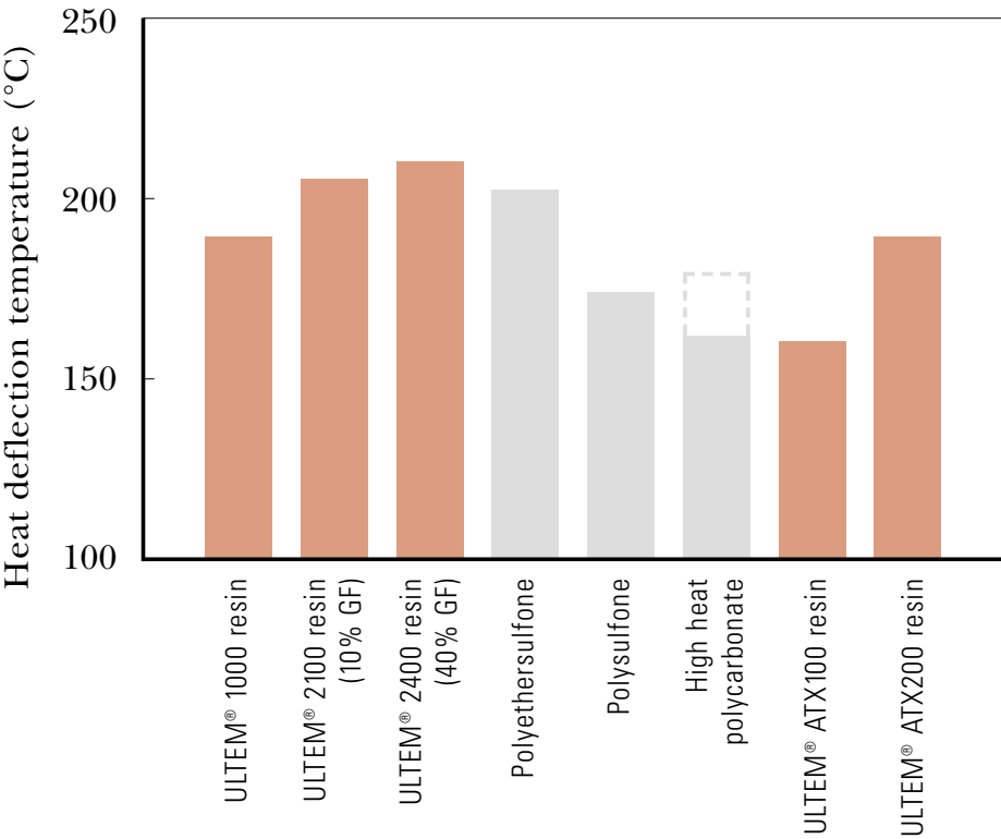
■ FIGURE 4-2 Heat Deflection Temperature (HDT/Ae 1.80 MPa)
