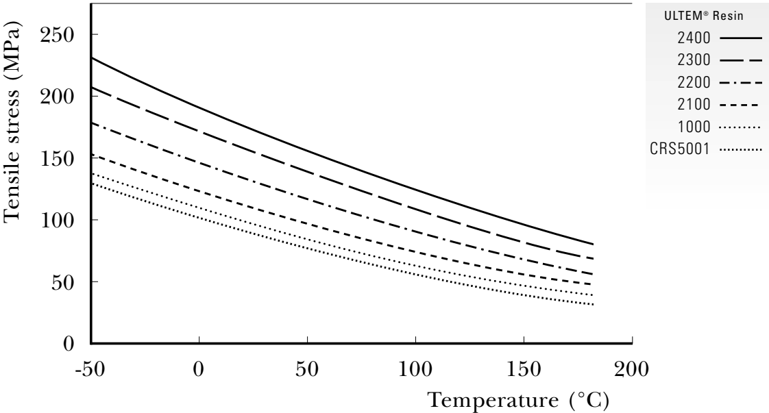
FIGURE 4-5 Tensile stress as a function of temperature
