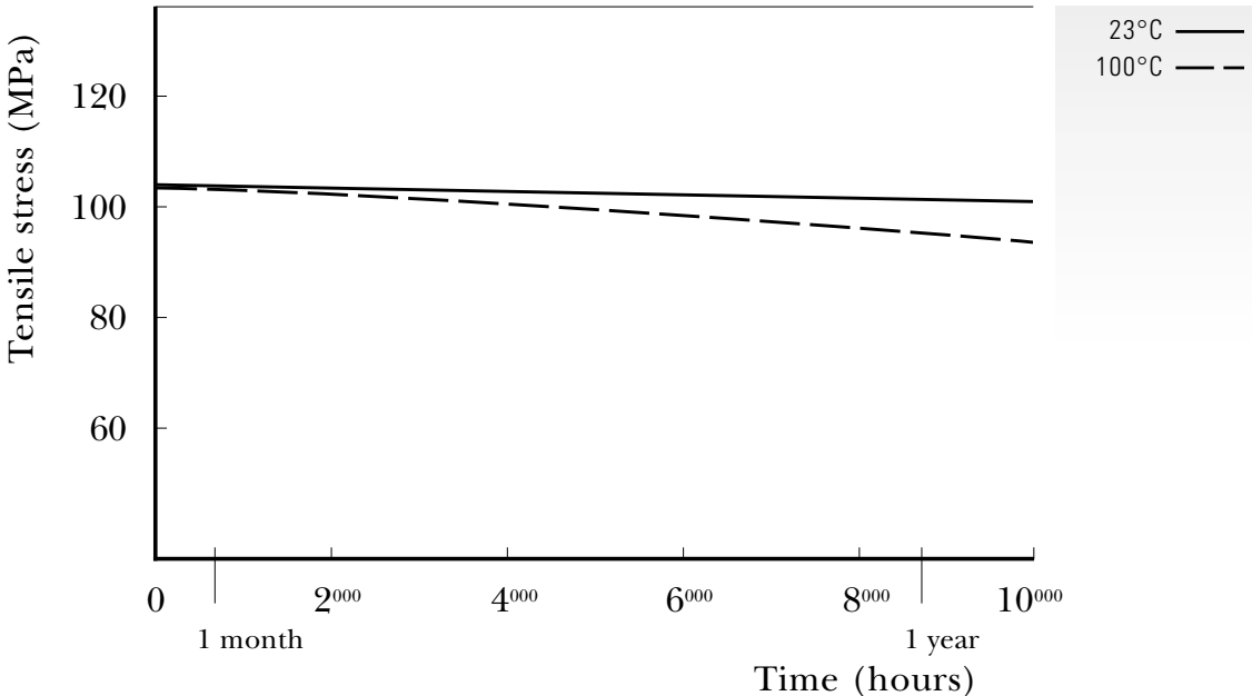
■ FIGURE 4-17 Effect of water exposure on tensile stress of ULTEM® 1000 resin
